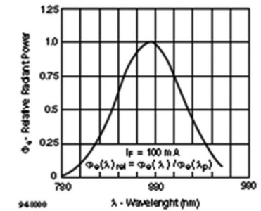
Fig. 9- Relative Radiant Power vs. Wavelength
